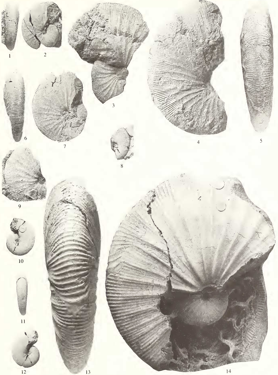
KENNEDY and HENDERSON, Phylloceras ( Neophylloceras )
